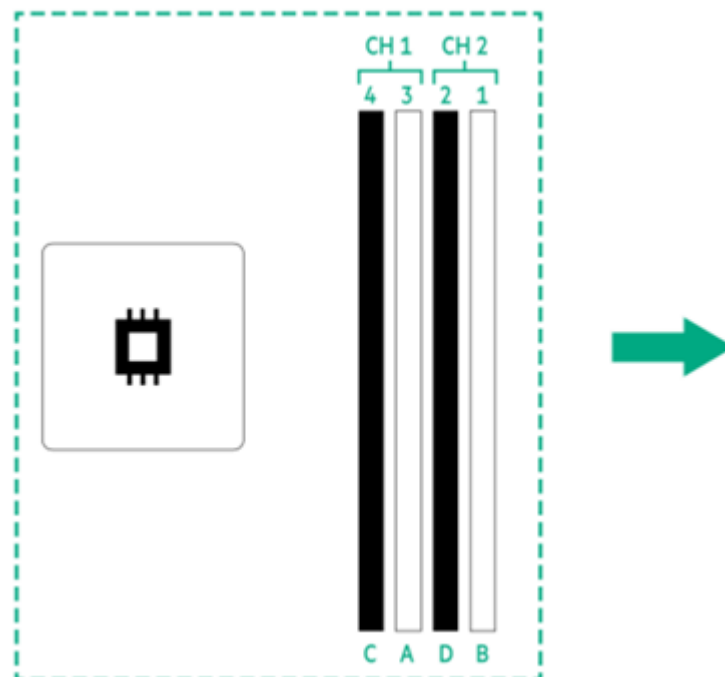
HPE ProLiant ML30 Gen10 Plus server memory slots
